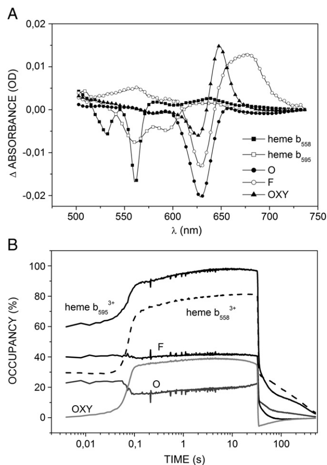
Fig. 3. A: Optical components (normalized to 1 \mu M enzyme): “heme b 558 ” = [Fe b558 3+ ] - minus-[Fe b558 2+ ]; “heme b 595 ” = [Fe b595 3+ ] - minus-[Fe b595 2+ ]; “ O ” = [Fe d 3+ ] - minus-[Fe d 2+ ]; “ F ” = [Fe d 4+ + O 2 - ] - minus-[Fe d 2+ ]; “ OXY ” = [Fe d 2+ - O 2 ] - minus-[Fe d 2+ ]. B: Percent occupancy of the optical species depicted in A, as obtained from the analysis of the spectra in the bottom panel of Fig. 2.
