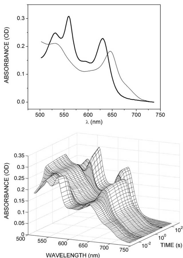
Fig. 2. Top: Absorption spectra of 10 \mu M cyt bd , “as isolated” (thin line) and in the fully reduced state (thick line). Bottom: Time-resolved absorption spectra collected up to 500 s after stopped-flow mixing O 2 -equilibrated buffer with cyt bd , pre-reduced by DTT and Q 1 . Concentrations after mixing: 10 \mu M enzyme; 5 mM DTT; 600 \mu M Q 1 . T = 20 °C.
