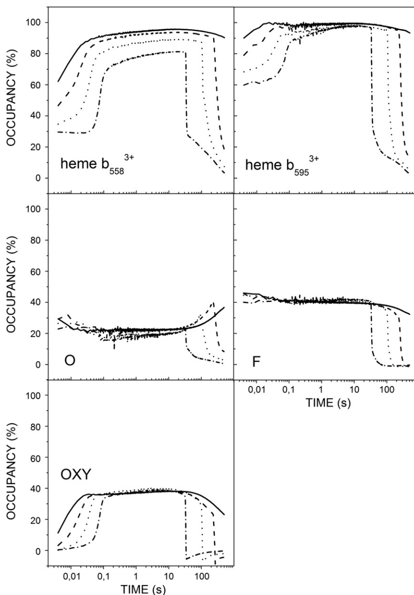
Fig. 5. Percent occupancy of each optical component as measured with cyt bd in turnover at increasing [Q 1 ]. Concentrations after mixing: 10 μM enzyme; 5 mM DTT; 50 μM (solid), 150 μM (dashed), 300 μM (dotted) or 600 μM (dash-dotted) Q 1 .
